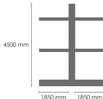
Storage rack with 3/2 floors (N-527533)
