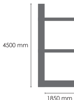
Storage rack with 3/1 floors (N-527532)
