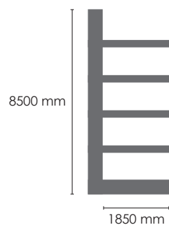
Storage rack with 5/1 floors (N-527582)
