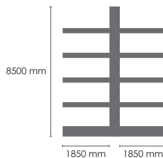
Storage rack with 5/2 floors (N-527583)
